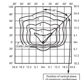
BXSPC**4MEF30K-UL w/XA-SP1BLS Mounting Height: 25' (7.6m) A.F.G. Initial Delivered Lumens: 8,687 Initial FC at grade
